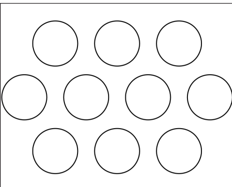
PATTERN 128 .500" Round | .688" Centers | 48% Open Area
