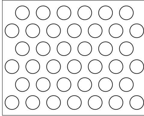
PATTERN 121 .250" Round | .375" Centers | 40% Open Area
