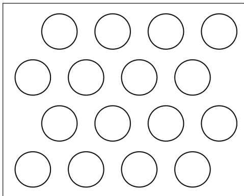
PATTERN 125 .375" Round | .563" Centers | 40% Open Area
