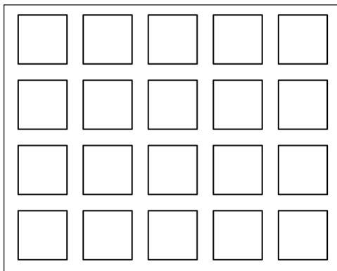
PATTERN 202 .375" Square | .500" Centers | 56% Open Area
