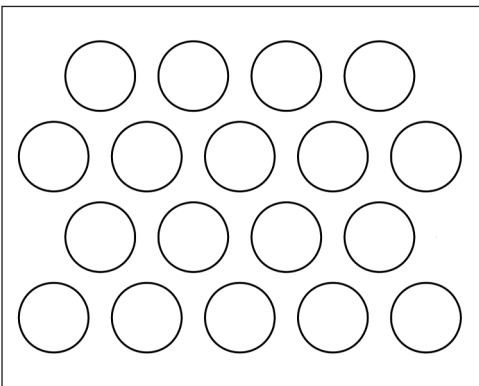
PATTERN 124 .375" Round | .500" Centers | 51% Open Area
