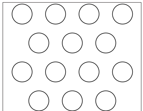
PATTERN 126 .375" Round | .625" Centers | 33% Open Area
