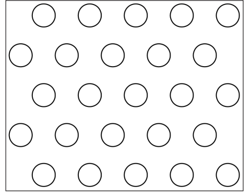
PATTERN 123 .250" Round | .500" Centers | 23% Open Area
