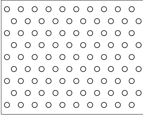
PATTERN 111 .094" Round | .250" Centers | 13% Open Area
