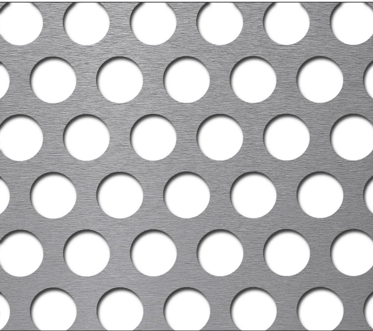
PATTERN 128 .500" Round | .688" Centers | 48% Open Area
