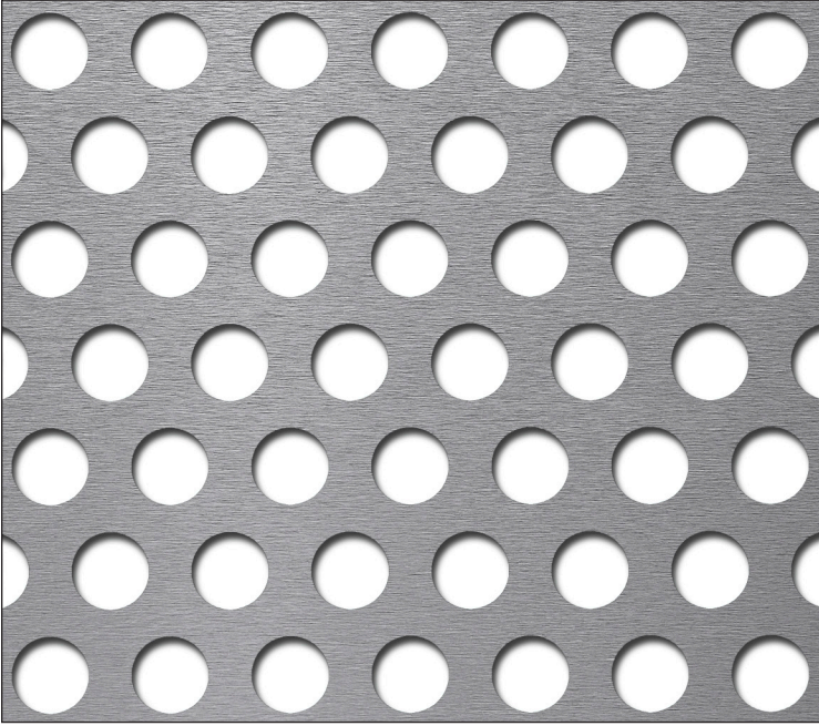
PATTERN 125 .375" Round | .563" Centers | 40% Open Area
