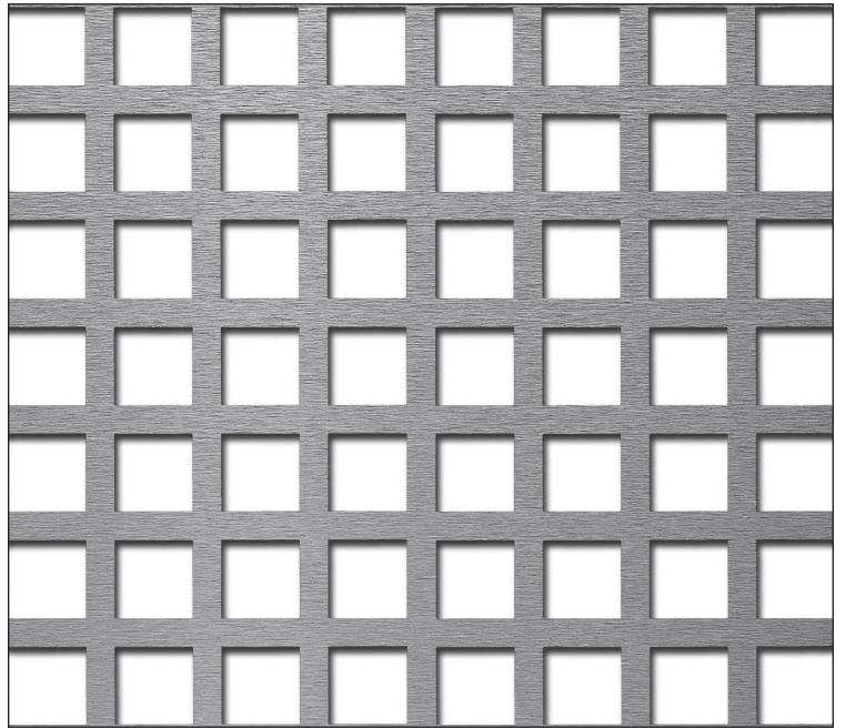
PATTERN 202 .375" Square | .500" Centers | 56% Open Area
